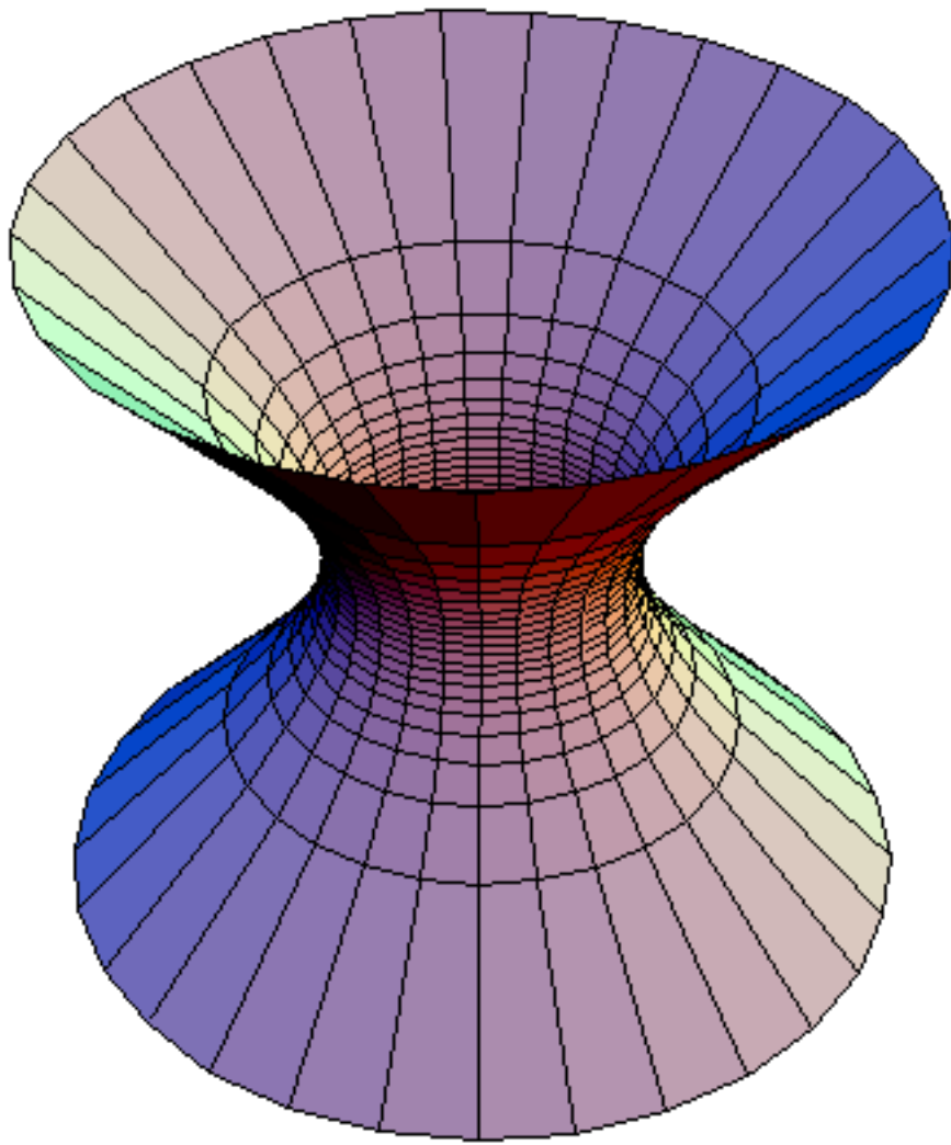
Hyperboloid
