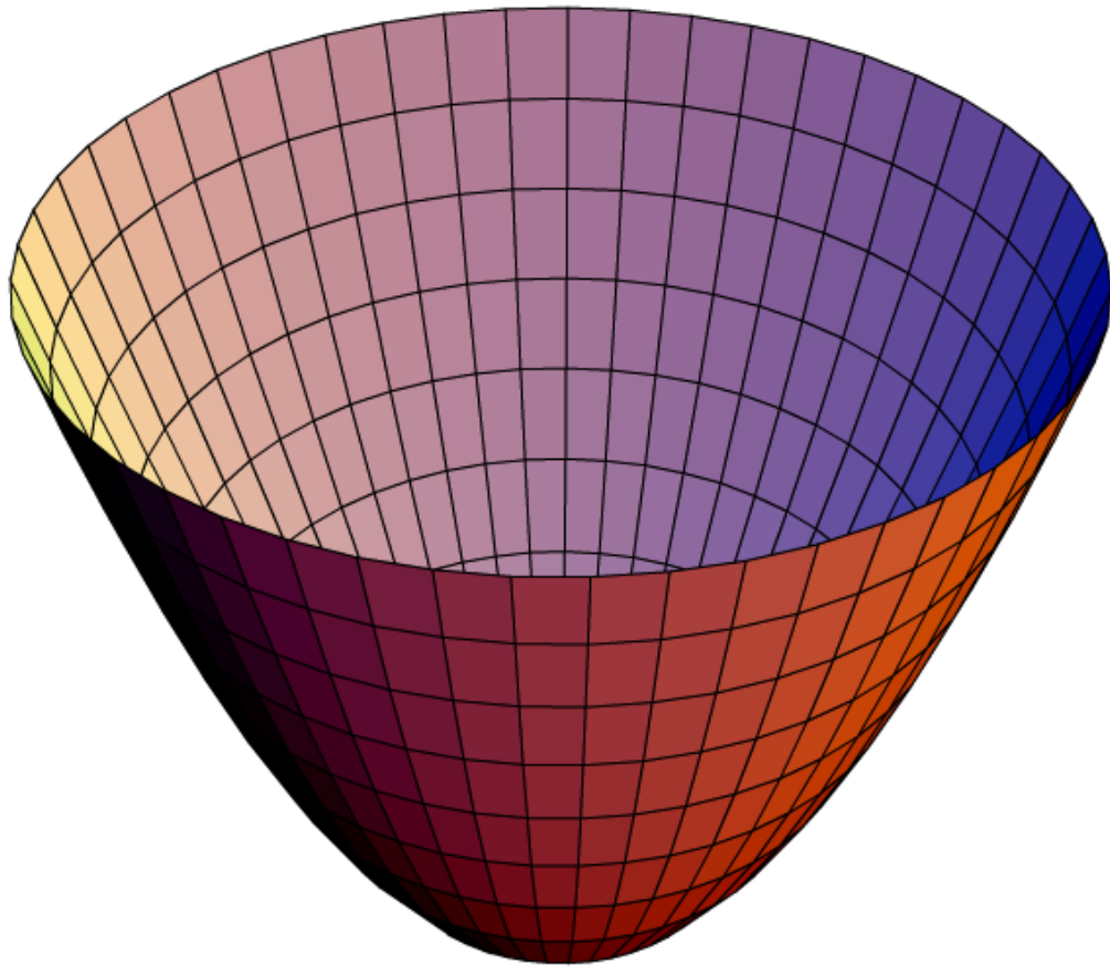
Paraboloid
